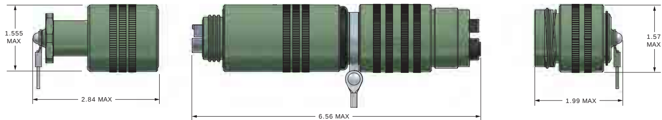
TFOCA-to-TFOCA-II® Adapter
