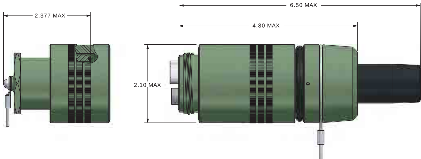
FS5H1000 TFOCA-III® Plug
